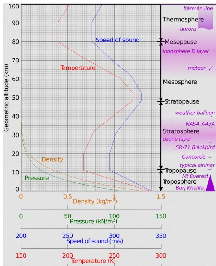
Figure 47: Earth's Atmospheric Density/Temperature 51
