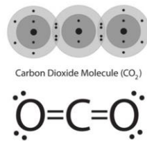
Figure 49: CO 2 Bonds and Configuration
